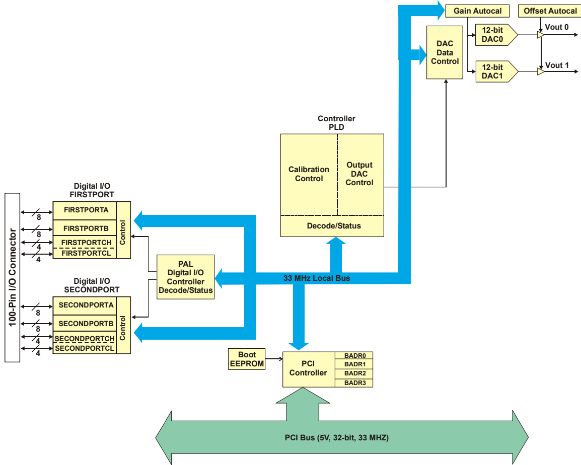
Figure 1-1. PCI-DDA02/12 functional block diagram
